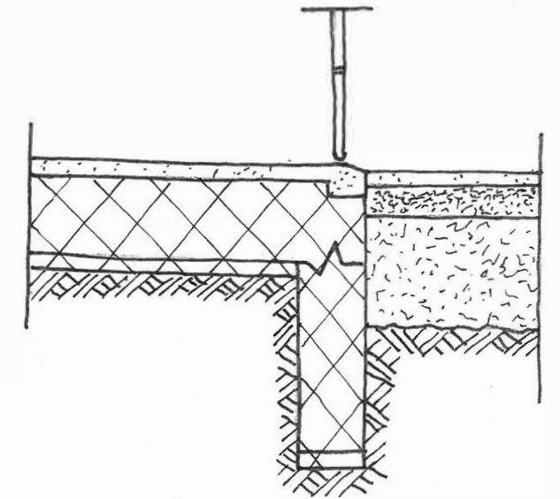
DETAIL GARAGENSOCKEL MST. 1:20
